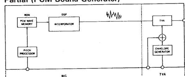
Partial (PCM Sound Generator)
