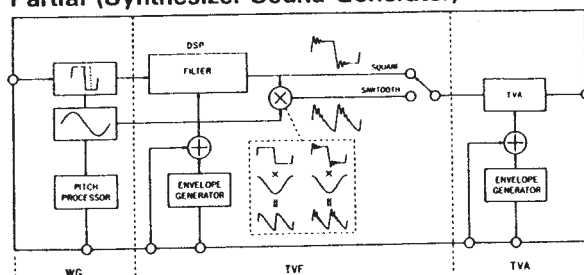
Partial (Synthesizer Sound Generator)
